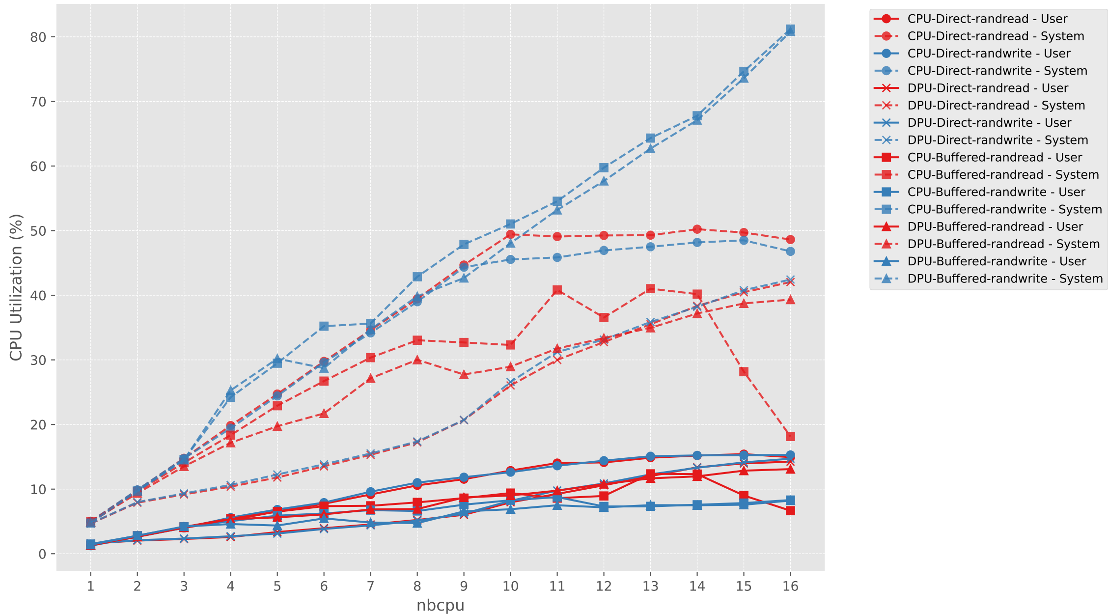
CPU Utilization vs nbcpu (CPU vs DPU, Direct vs Buffered)
